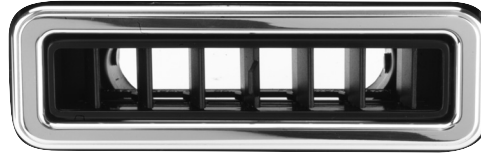
49063-VUQ Streamline louver. Smooth polished aluminum trim. Face size 1.75"x 4.875"
