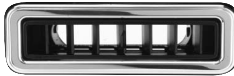
49063-VUQ Streamline louver. Smooth polished aluminum trim. Face size 1.75"x 4.875"
