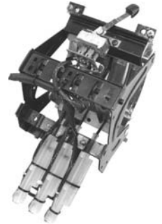
OEM '55-'56 Chevy control with supplied Electronic Cable Converters™ installed from Gen IV kit.
