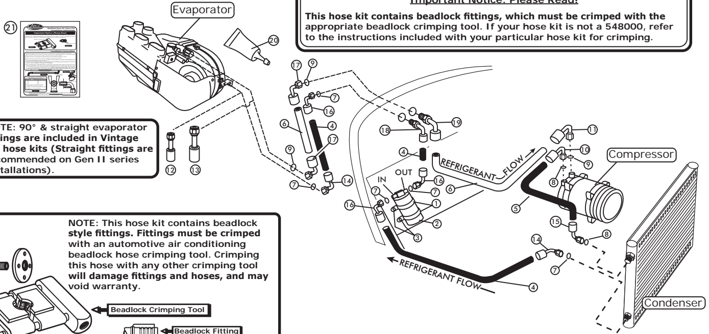
Beadlock Fitting
